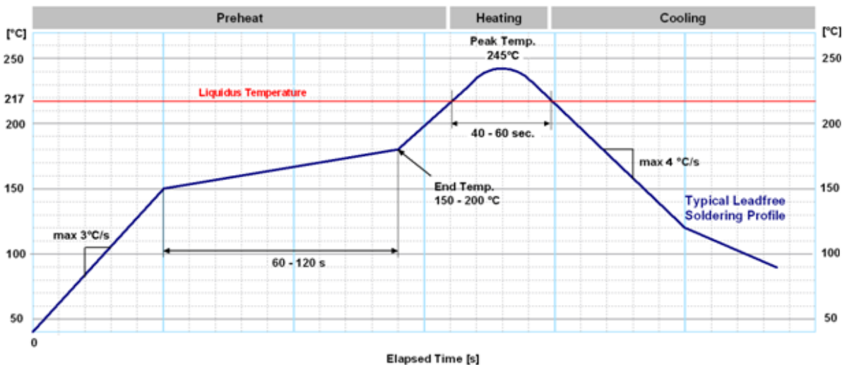
Figure 27: Soldering profile
