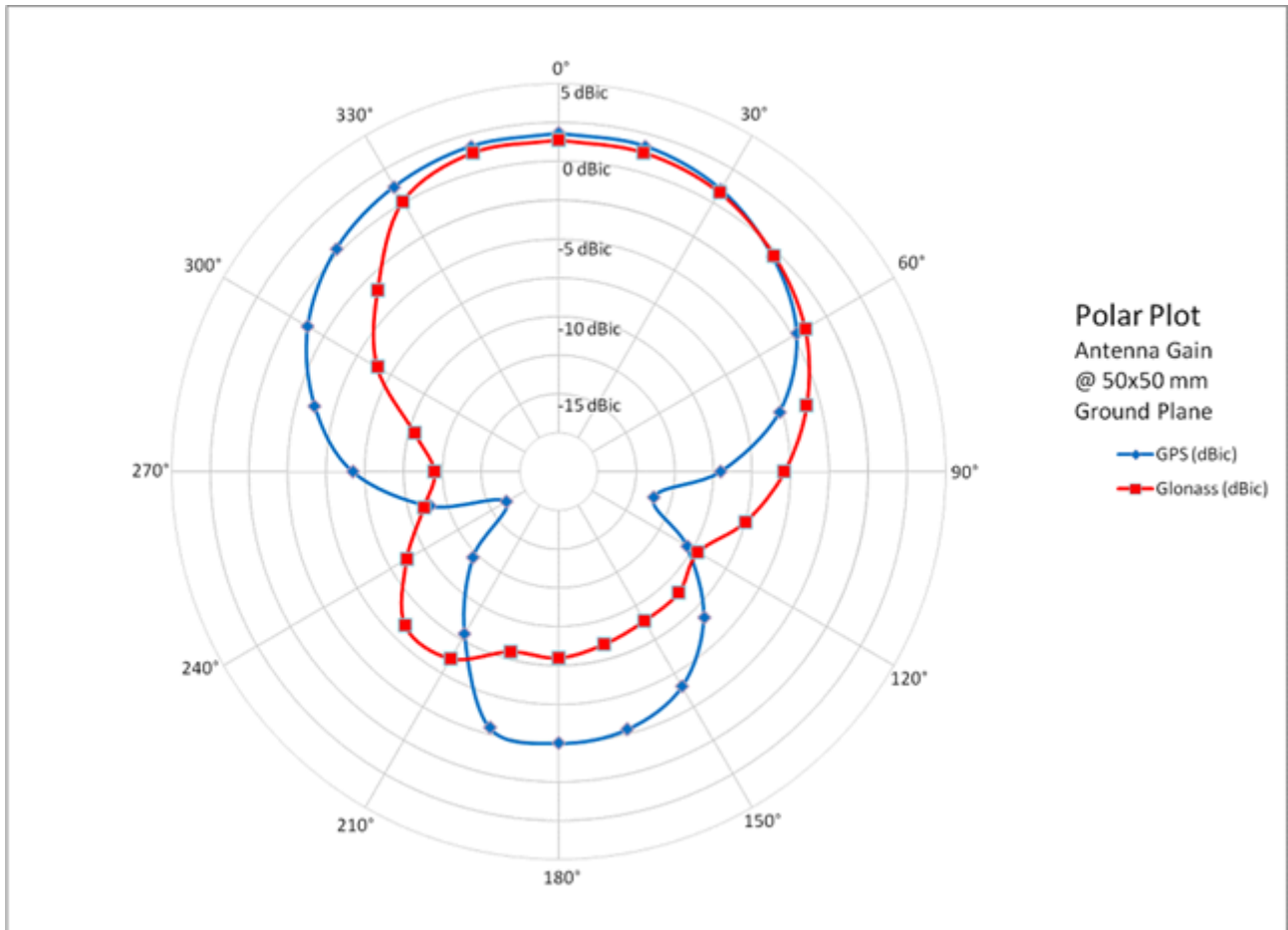
Figure 20: SAM-M10Q antenna RHCP gain pattern in free space at GPS and GLONASS bands. Measured on a 50 x 50 mm 2 ground plane.
