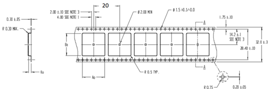
Figure 26: Tape dimensions (mm)
